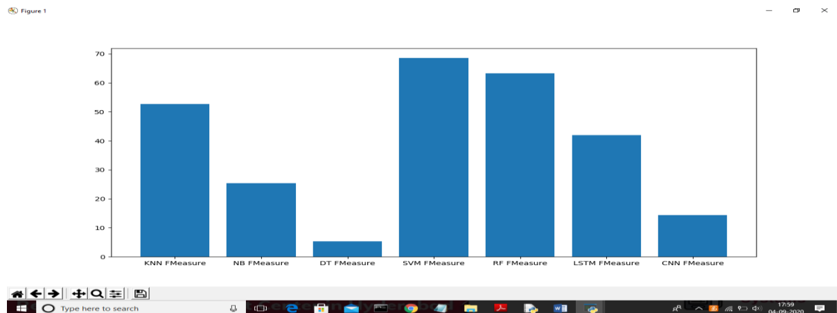
Figure 5 Comparison of FMeasure
